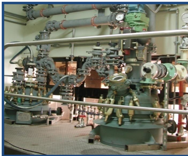
50 L Glass Lined Reactor
